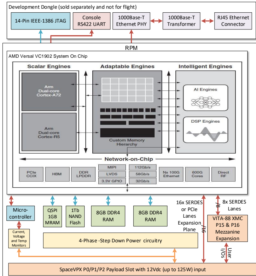
Figure 1. Frontgrade RPM-PS Block Diagram
